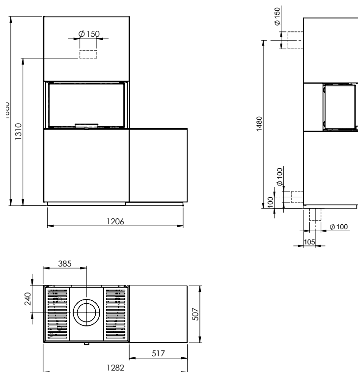
FIG 4 MONACO II HIGH + WOOD SHELF/Q-34 UL = CHIMNEY/AIR/MM
