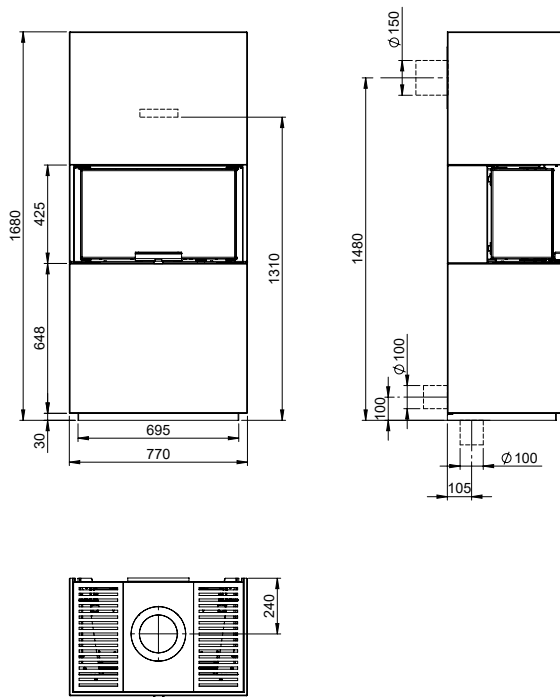
FIG 3 MONACO II HIGH/Q-34 UL = CHIMNEY/AIR/MM
