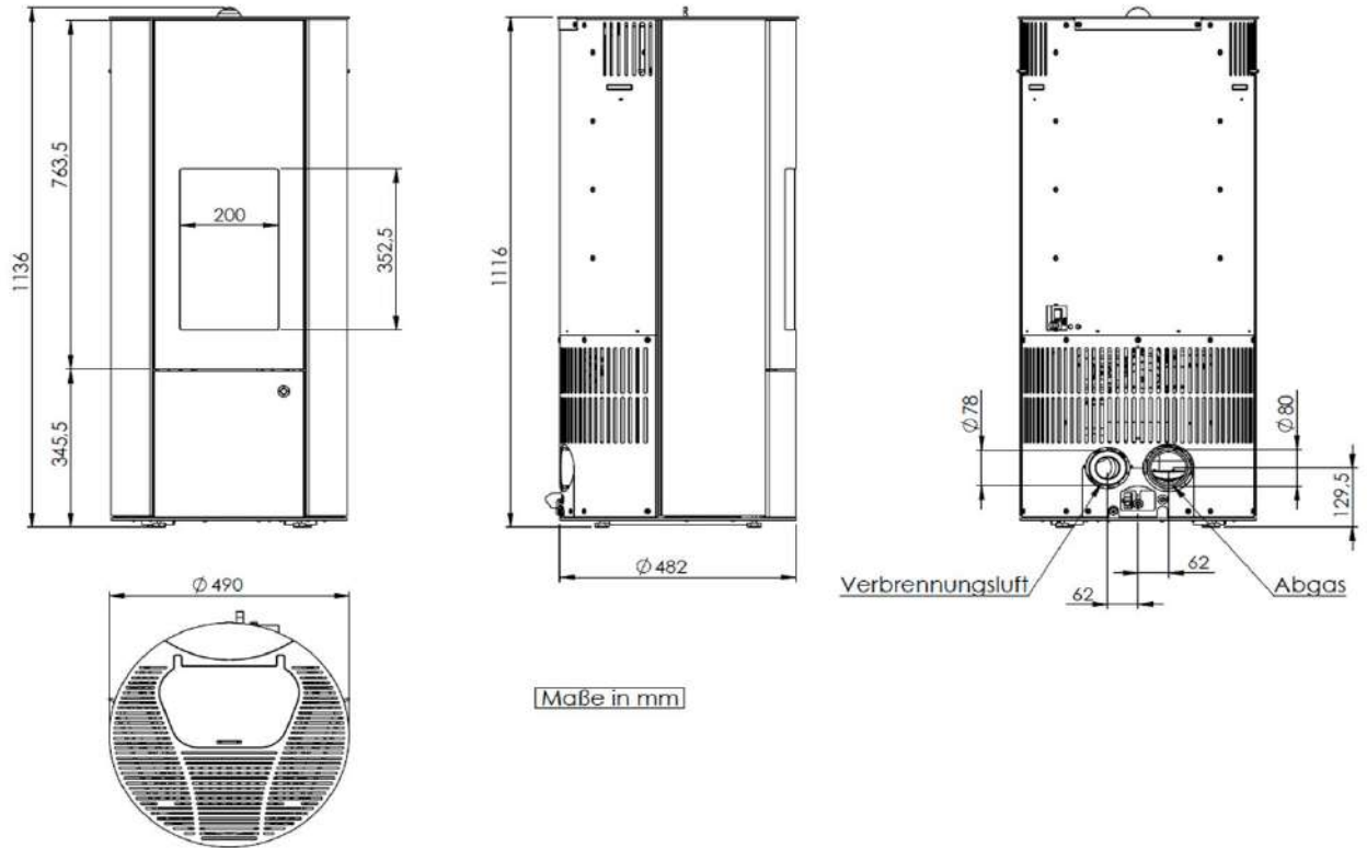
Olsberg Inara 6kW
